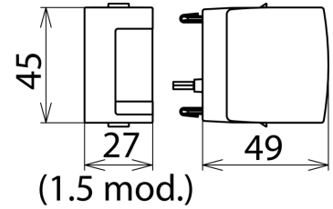
Dimension drawing DG MOD E PV SCI 750
