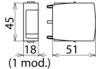
Dimension drawing DG MOD PV 300
