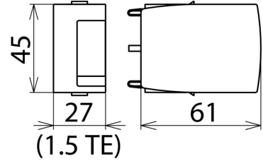
Dimension drawing DG MOD E H LI 275
