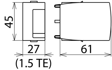
Dimension drawing DG MOD E H LI 1000
