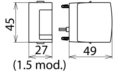
Dimension drawing DG MOD E DC 60
