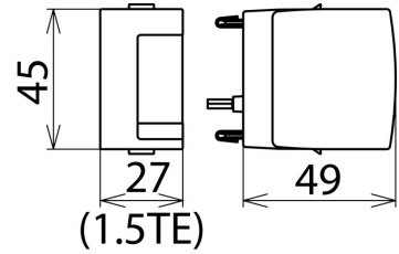
Dimension drawing DG MOD E DC 900
