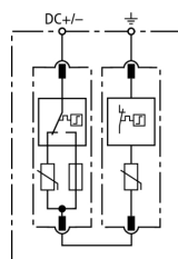
Basic circuit diagram DG S PV SCI 150
