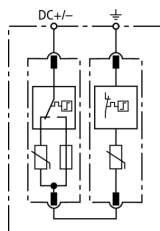
Basic circuit diagram DG S PV SCI 600
