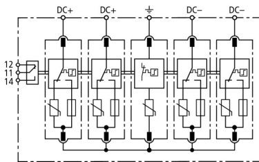
Basic circuit diagram DG M PV2 SCI 1000 FM
