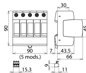
Dimension drawing DG M PV2 SCI 1000 FM
