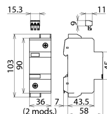
Dimension drawing DG 1000 FM
