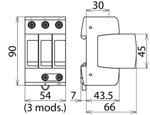
Dimension drawing DG M TNC 275
