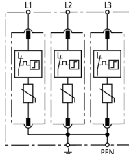
Basic circuit diagram DG M TNC 385
