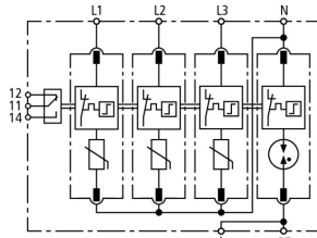
Basic circuit diagram DG M TT 150 FM
