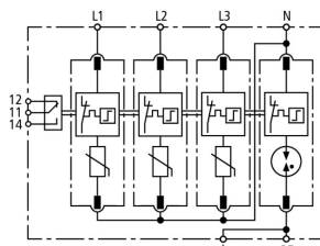
Basic circuit diagram DG M TT 385 FM
