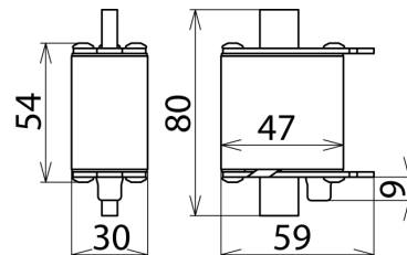
Dimension drawing VA NH00 280
