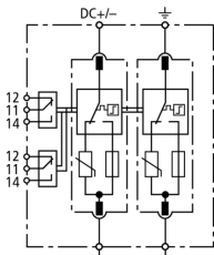
Basic circuit diagram DG SE PV SCI 1500 FM
