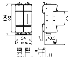
Dimension drawing DG SE PV SCI 1500 FM
