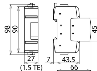
Dimension drawing DG SE DC 900
