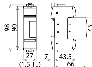
Dimension drawing DG SE DC 60
