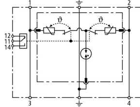
Basic circuit diagram DR M 2P 60 FM
