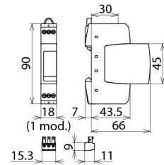
Dimension drawing DR M 2P 60 FM
