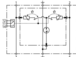
Basic circuit diagram DR M 2P 75 FM
