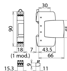
Dimension drawing DR M 2P 150 FM
