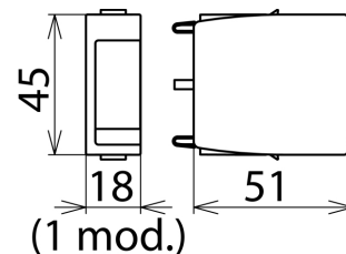
Dimension drawing DR MOD 30
