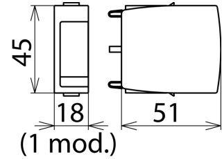
Dimension drawing DR MOD 150
