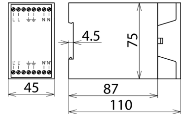
Dimension drawing NF 10
