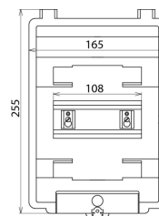
Dimension drawing IGA 6 IP54
