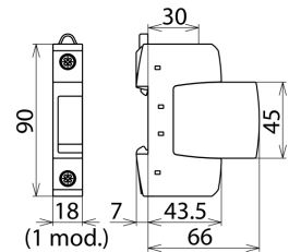
Dimension drawing DK 25
