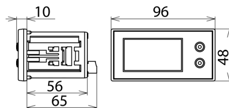
Dimension drawing DPAN L
