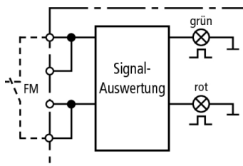
Basic circuit diagram DPAN L
